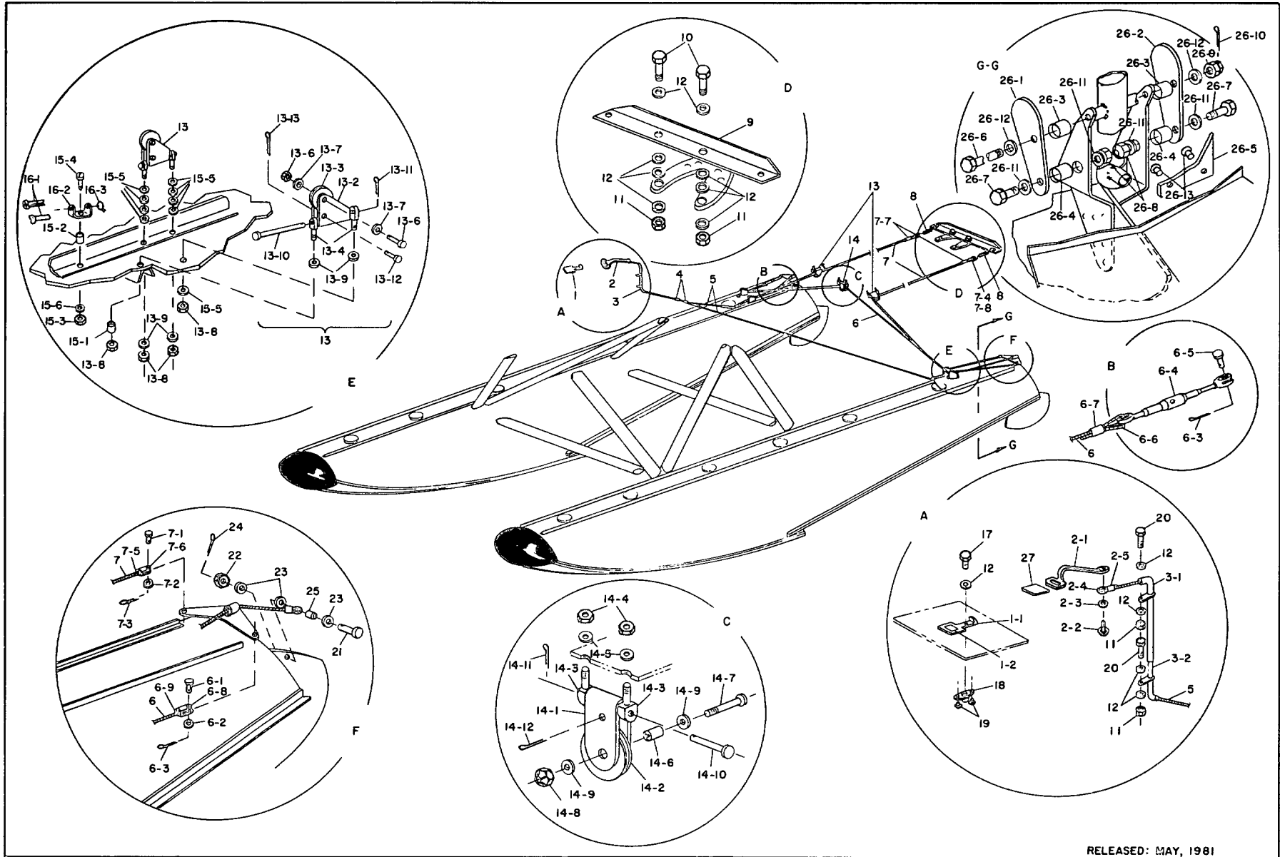
FIGURE 2. EDO WATER RUDDER CONTROLS MODEL 089-15 FOR EDO 089/089A2000 FLOATS ON CESSNA 172 (TUBULAR GEAR)
