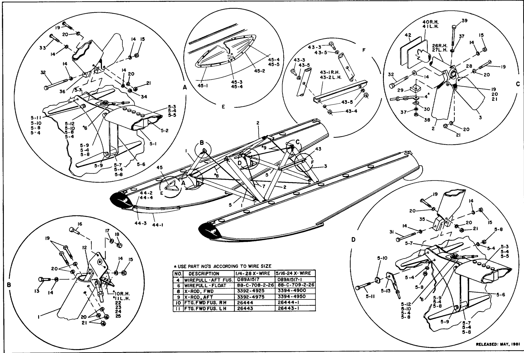
FIGURE 1. EDO ATTACHMENT GEAR MODEL 089-15 FOR EDO 089/089A2000 FLOATS ON CESSNA 172 (TUBULAR GEAR)
