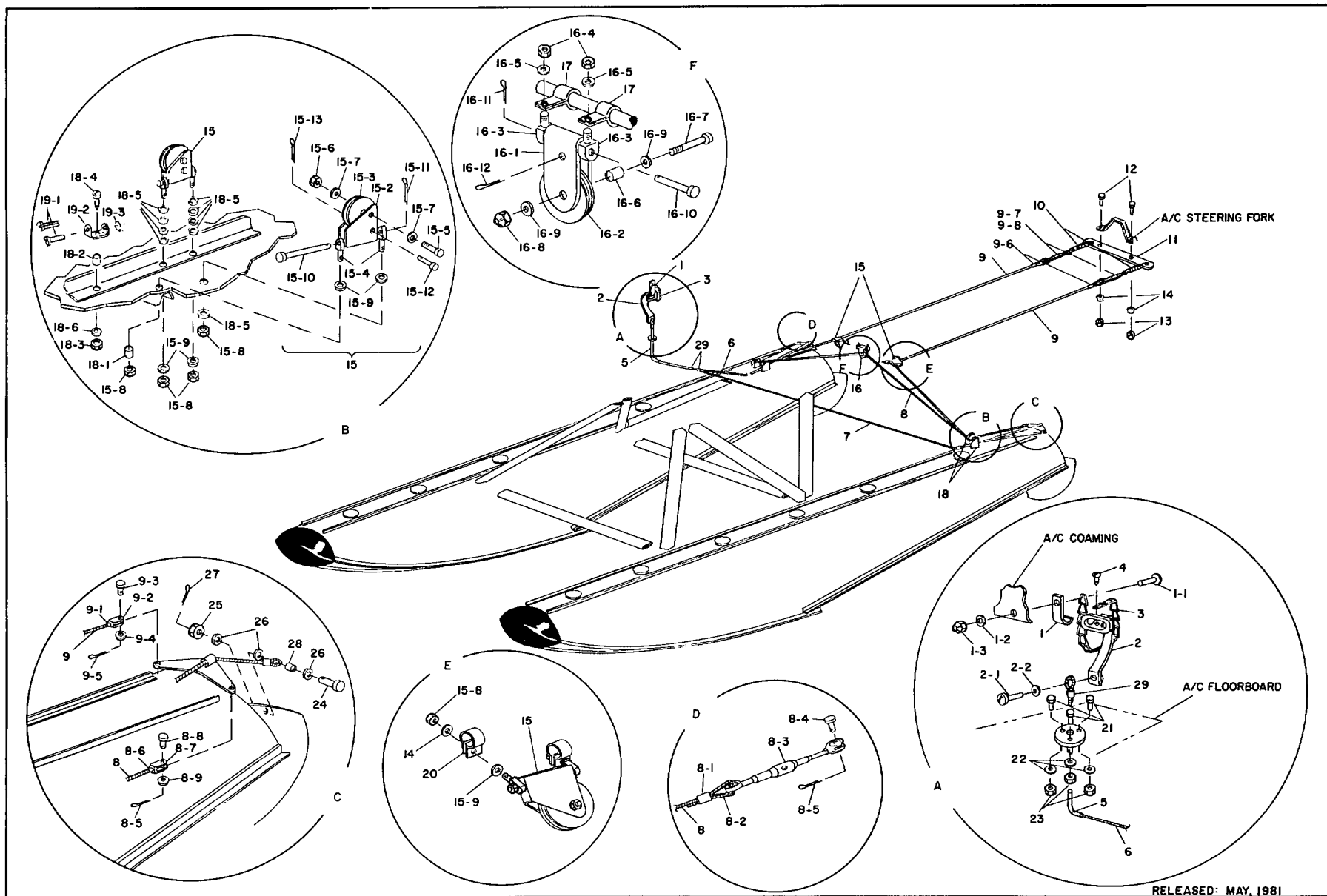
FIGURE 2. EDO WATER RUDDER CONTROLS MODEL O89-26 FOR EDO O89/O89A2000 FLOATS ON PIPER PA-18 (EXTRUDED GEAR)
