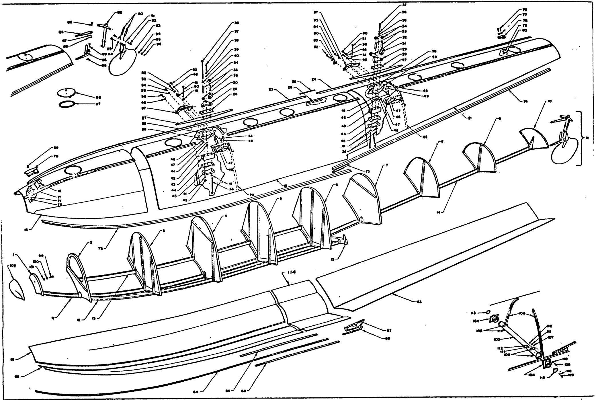
FIGURE 1 - EDO MODEL 249-2870 FLOAT
