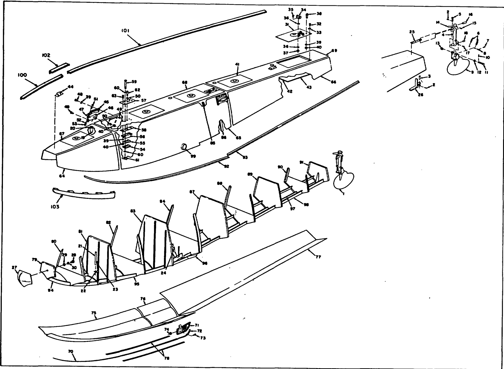
EDO MODEL 582-3430 FLOAT
