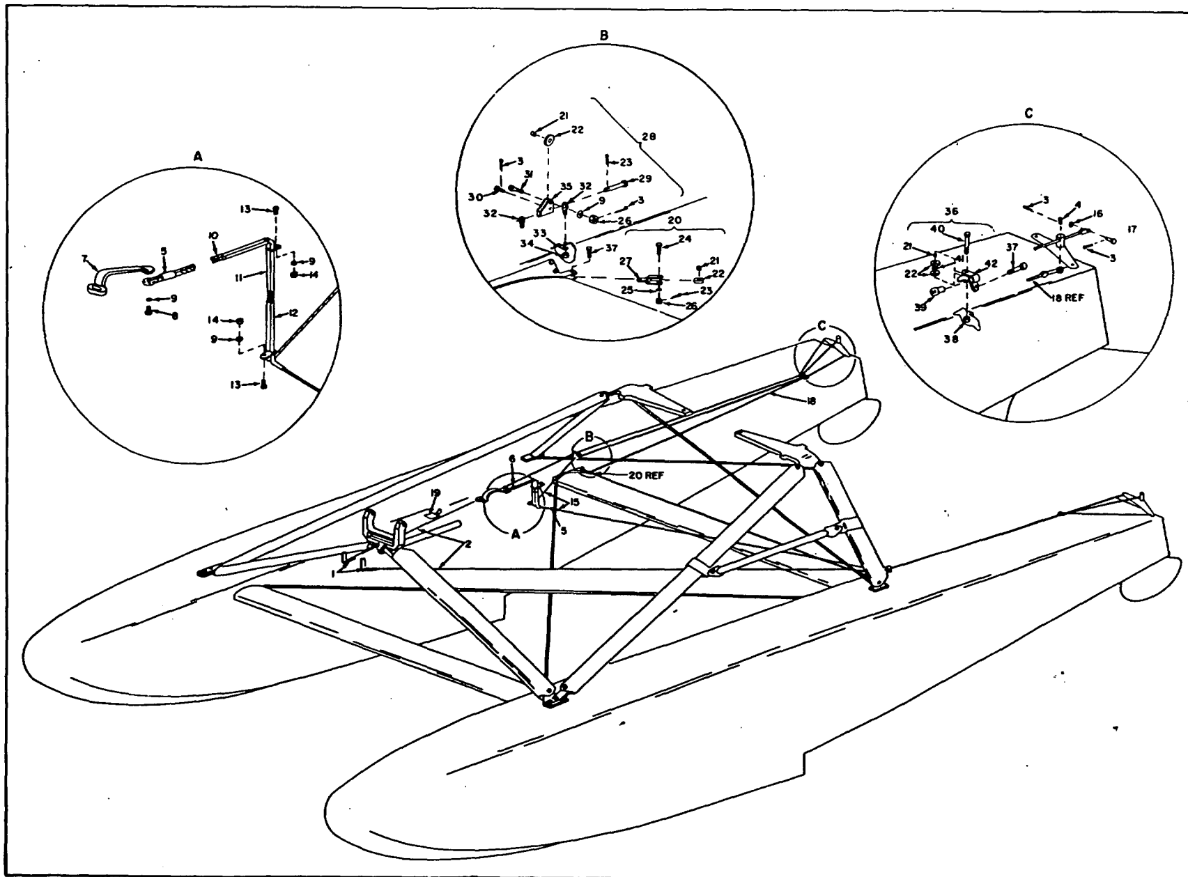
FIG. 2 EDO WATER RUDDER CONTROLS NO. 582-11 FOR 582-3430 FLOATS ON CESSNA 206
