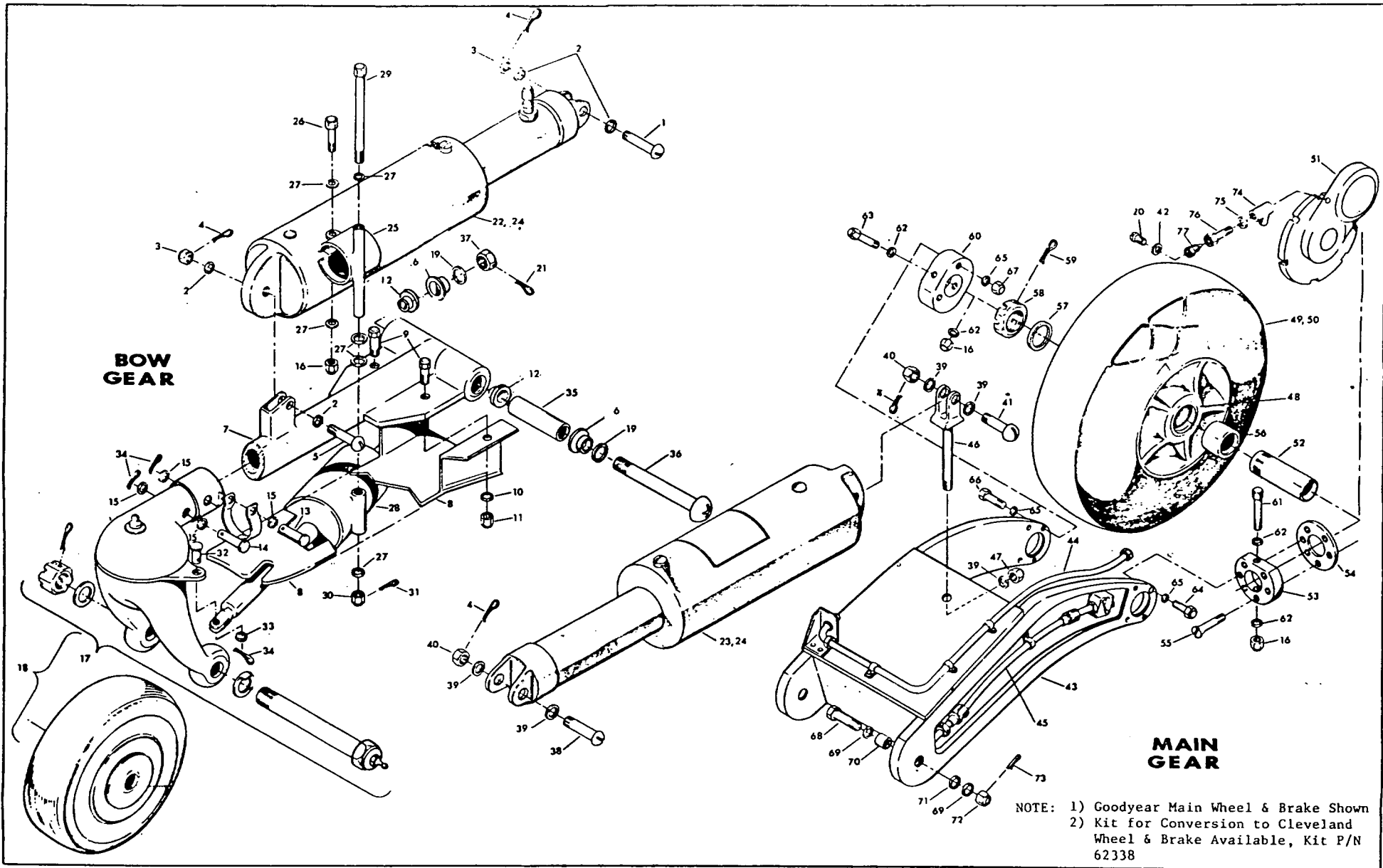
FIGURE 2. EDO BOW AND MAIN LANDING GEAR
