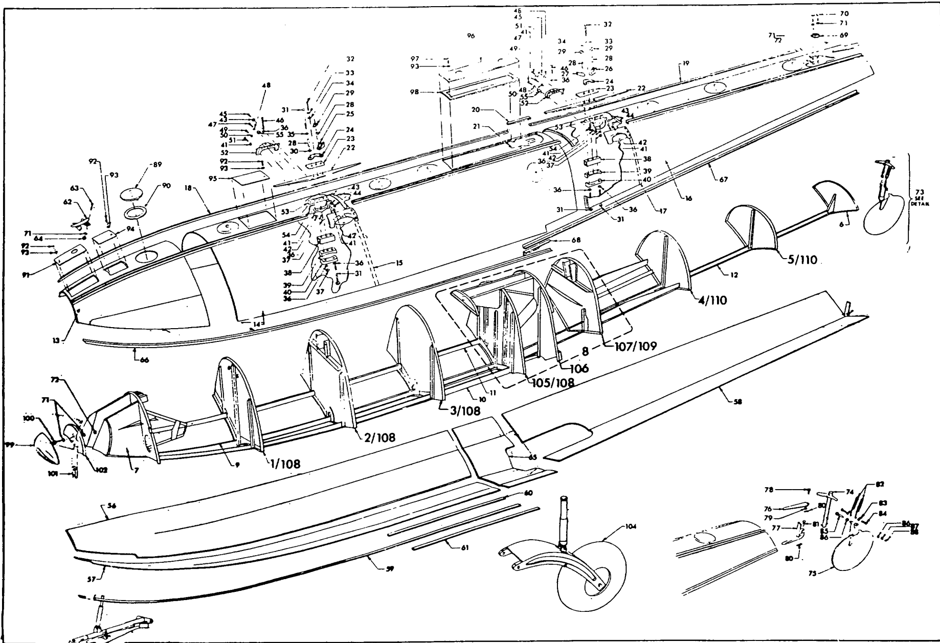
FIGURE 1. EDO MODEL 289-2700 FLOAT
